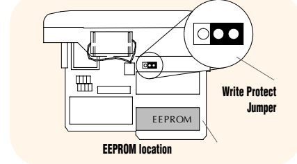
CPU Side View
