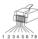
8-pin RJ45 Connector 8P8C
