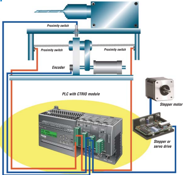
Multihead drill machine application
